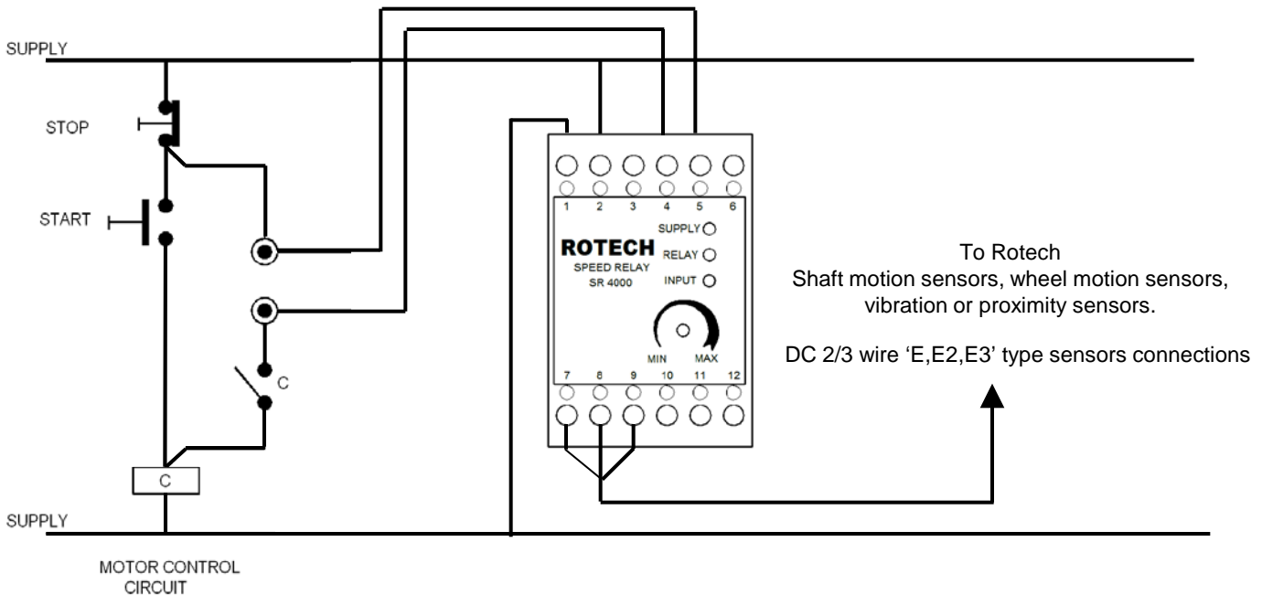
Typical installation shown for 110/120 V AC supply
